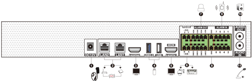
Rear panel
